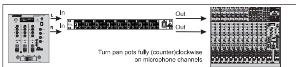
Fig. 3.2: DJ mixer → DI-box → mixer
